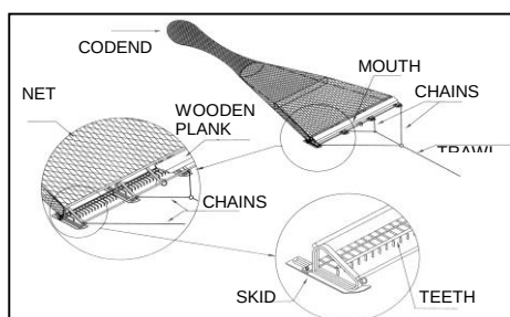
Scheme of rapido trawl used in GSA 17
