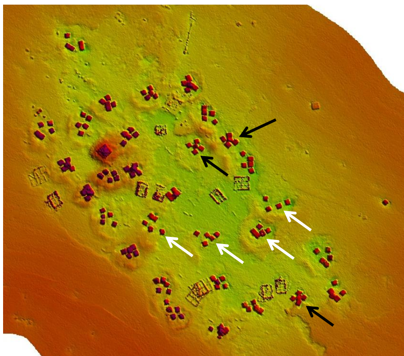
Fig. 24 – Italy: multibeam echosounder image of on artificial reef in the Adriatic Sea 21 years after deployment. Some reef sets have maintained their original structure (black arrows), while others have collapsed (white arrows) (courtesy of CNR-ISMAR Ancona).
