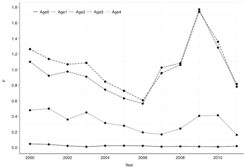
Figure 6.6: F by age estimated by the means of the LaRec-Shepherd VPA.
