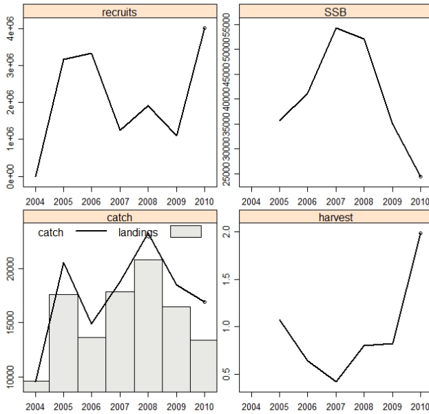
Figure 6.9: Time-series of horse mackerel population estimates of total stock in the Black Sea (FLR for Quantitative Fisheries Stock Assessment Analysis with terminal F=1.2 ): A. recruitment (line) and stock spawning biomass (SSB); B. landings (grey) and catch (line) (after Daskalov et al., 2011).
