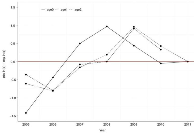
Figure 6.12: Observed \log(q) – Expexted \log(q) by age estimated by VPA analysis.
