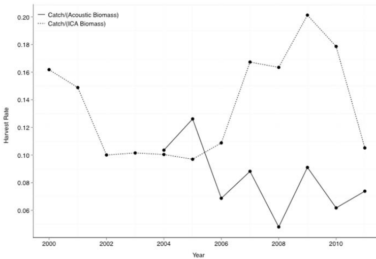
Figure 6.3: Harvest rate estimates ( C/B ) obtained from the mid-year ICA biomass (dashed line) and the acoustic biomass (full line).
