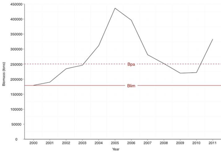
Figure 8.1: Mid year stock biomass and proposed reference points.
