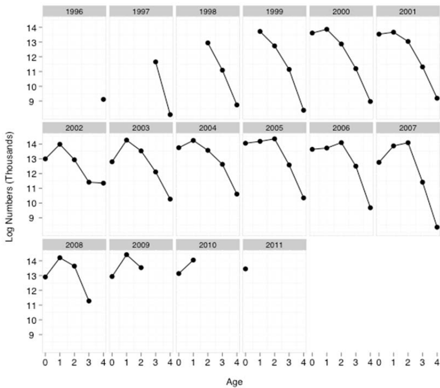
Figure 3.2.2: Log numbers at age (thousands) of the catch at age used in the assessment.
