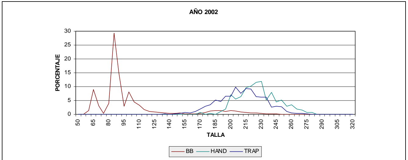
Figure 8. Length distributions of bluefin tuna caught by bait boat, hand line and trap (feeding migration) in the Strait of Gibraltar for year 2002.
