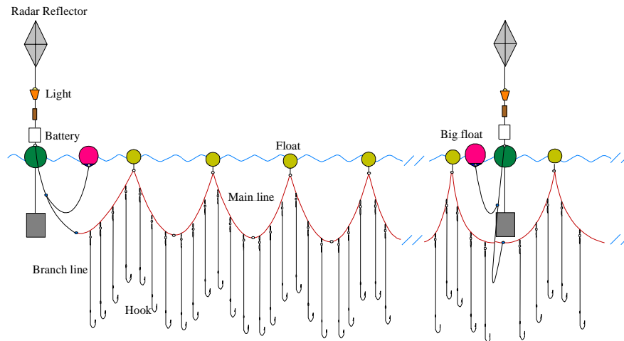
Figure 19. Diagram of surface longline targeting the albacore used by the Spanish fleet.
