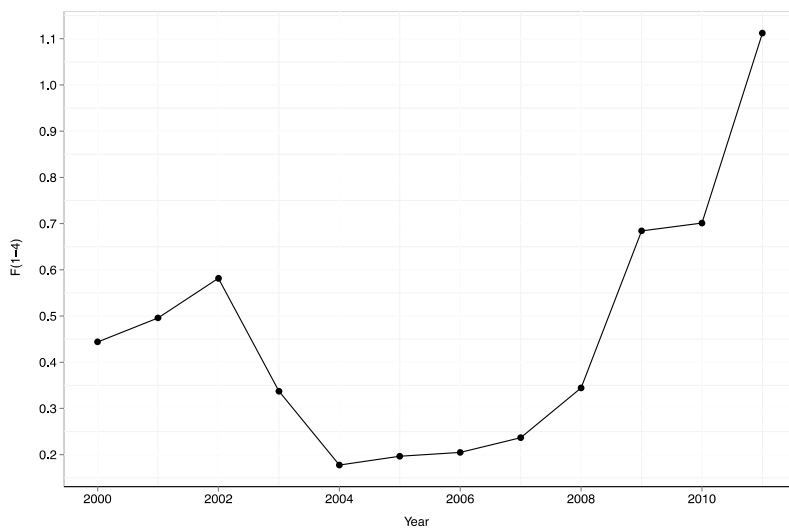
Figure 8.3: \bar{F}_{bar(1-4)} estimates.
